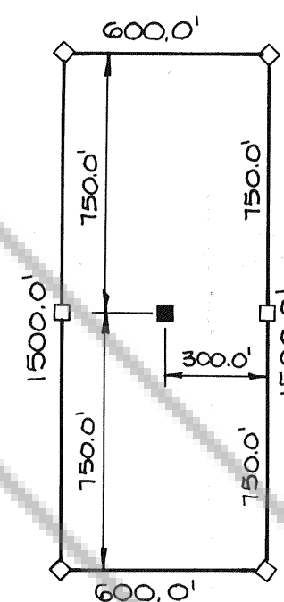
TYPICAL DIMENSIONING FOR CEDAR 1-13 LODE CLAIMS
