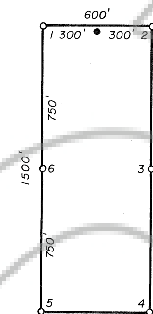
TYPICAL CLAIM DISCOVERY MONUMENT IS 20' FROM END LINE
