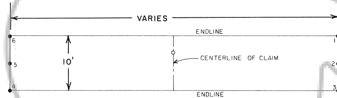
TYPICAL DIMENSIONS AND CORNER NUMBERING DETAIL NO SCALE (KL-4A IS NOT TYPICAL)
