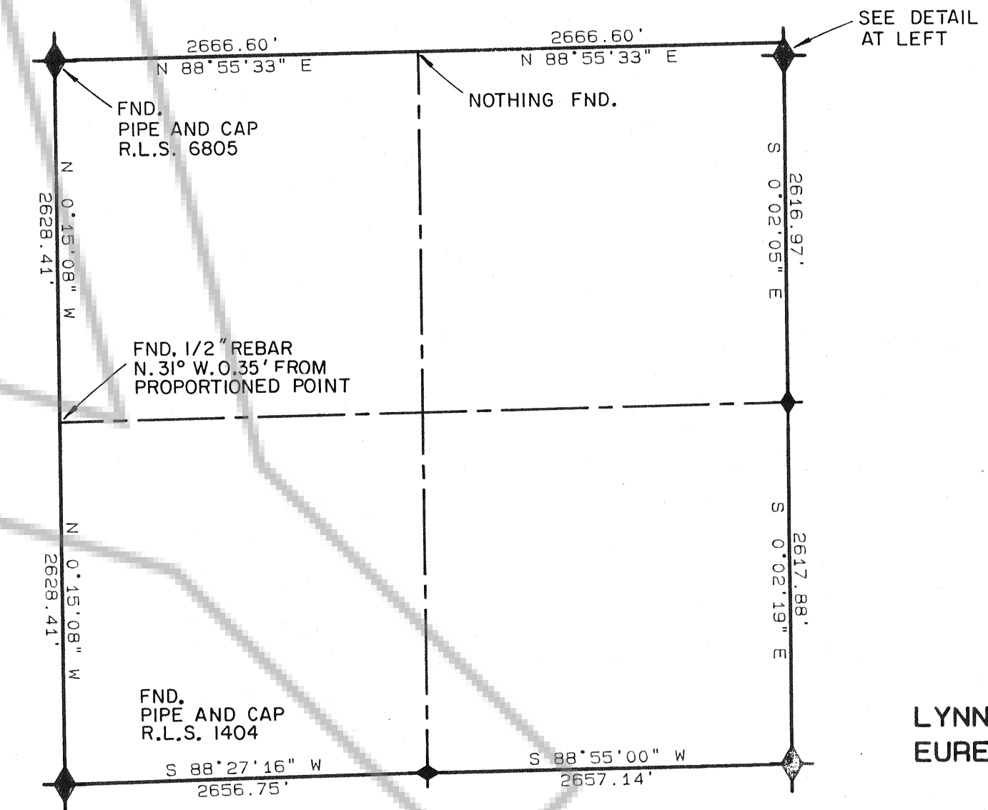
SECTION LINE DIMENSIONS FOR SEC. 36 (SCALE: 1" = 1000')
