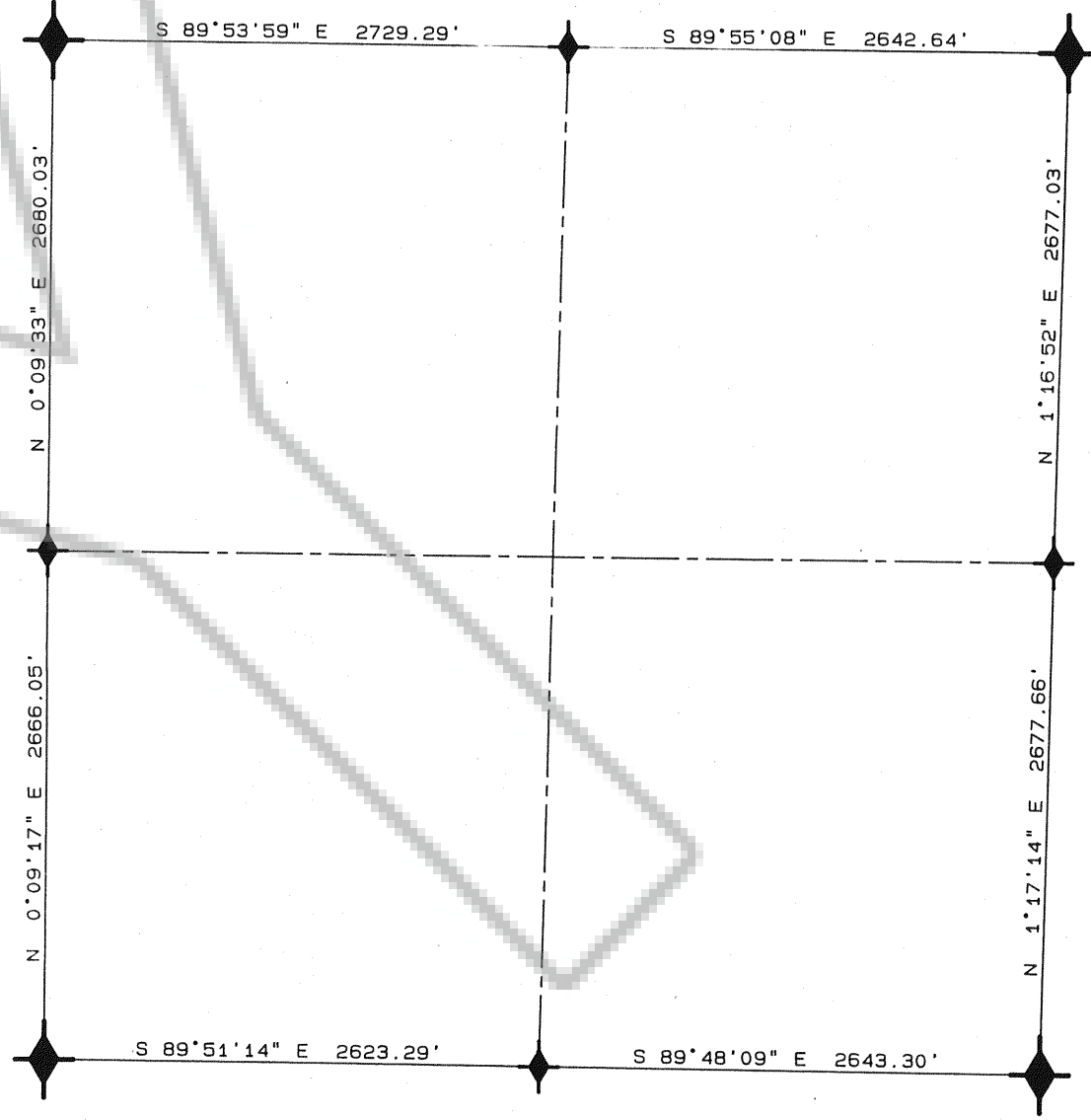
SECTION LINE DIMENSIONS FOR SEC. 30 (SCALE: 1" = 1000')
