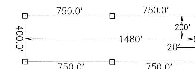
TYPICAL DIMENSIONING SOCK 1 & 24 LOCATION MONUMENT OCCURRING AT EITHER END OF CLAIM
