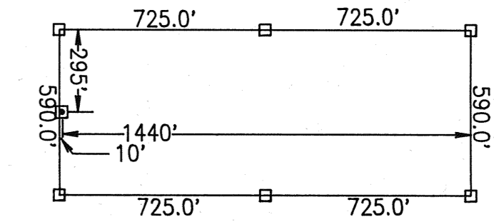
TYPICAL DIMENSIONING RING 19 - 36 LOCATION MONUMENT OCCURRING AT EITHER END OF CLAIM
