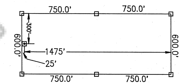
TYPICAL DIMENSIONING RING 1 - 18 LOCATION MONUMENT OCCURRING AT EITHER END OF CLAIM
