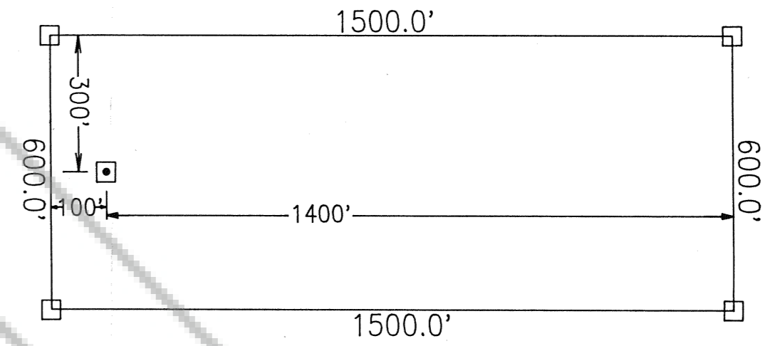
TYPICAL DIMENSIONING TRES 1-27 LOCATION MONUMENT OCCURRING AT EITHER END OF CLAIM
