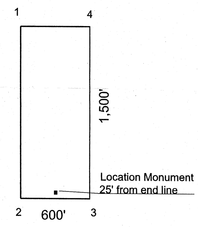
Typical Lode Mining Claim all corners marked by 1.5" X 1.5" X 4' wood posts
