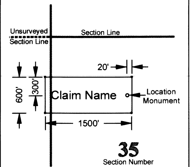
Typical Lode Mining Claim Not To Scale
